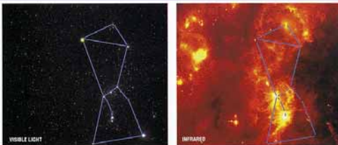
Photo by NASA/JPL/Caltech. Orion Constellation seen in visible and infrared light.
